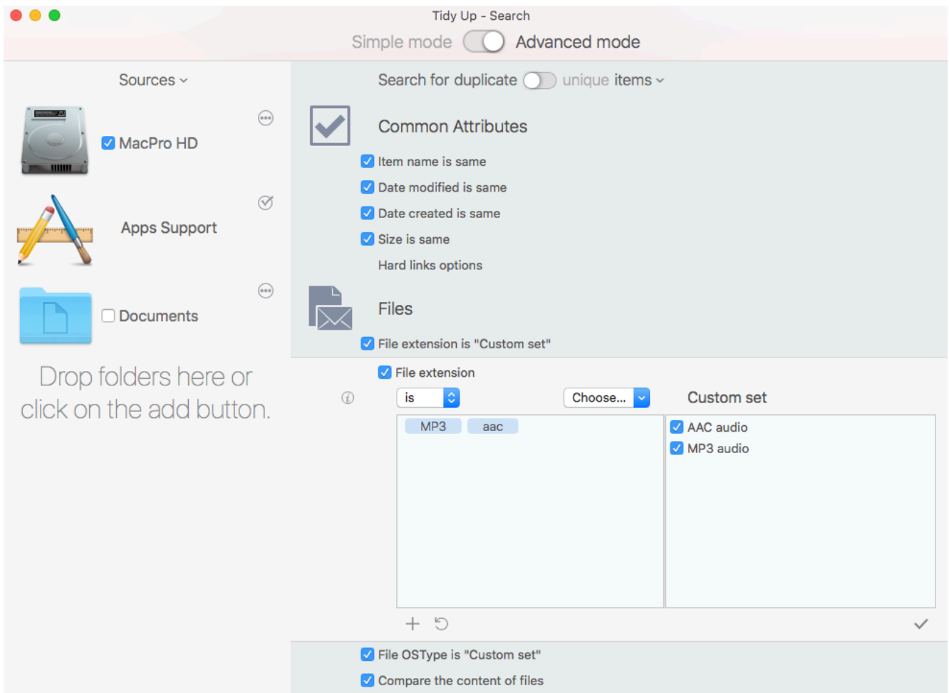
Figure 75: Search for duplicate MP3s and AACs (not in the Music library) by file attributes.
