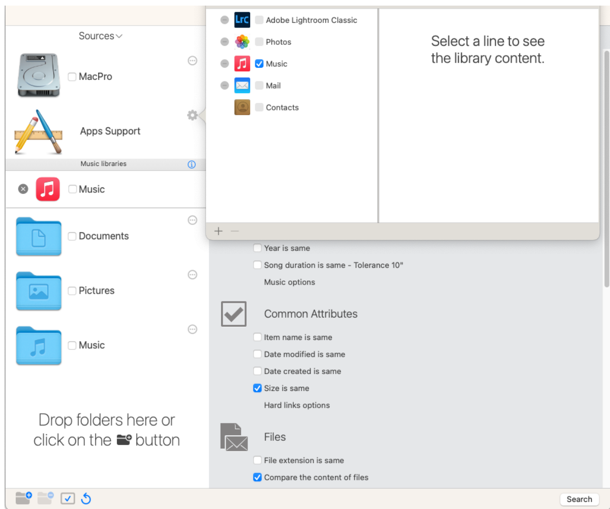
Figure 77: Search for duplicates in Music library.
