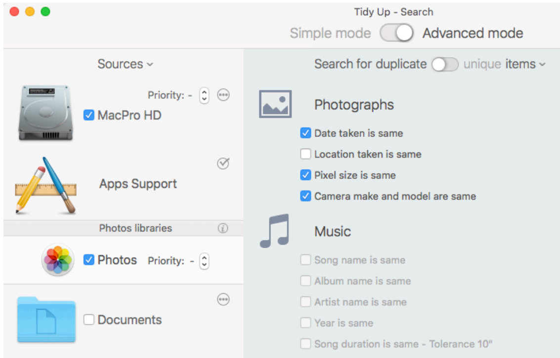
Figure 80: Search for similar images by the EXIF metadata.
