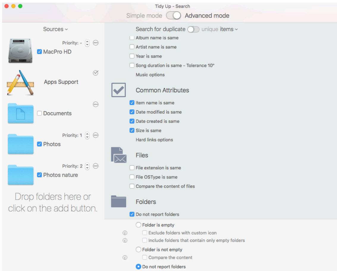
Figure 67: Search for similar files.
