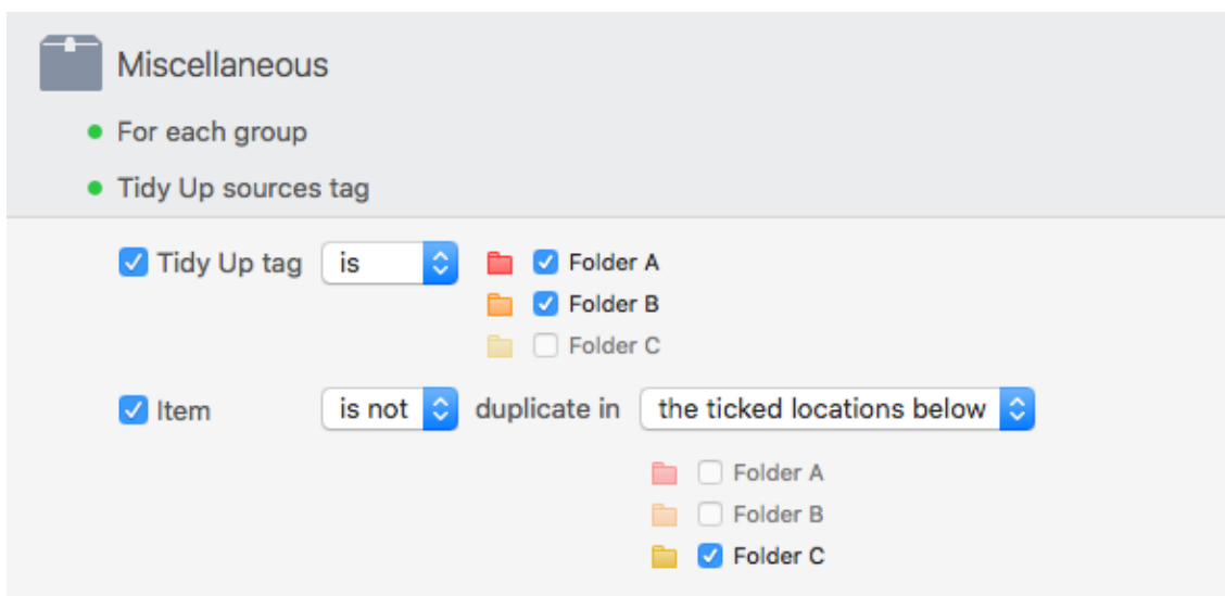
Figure 97: Remove all but one item of each duplicate group that reside in a specific location, but only if they are duplicates with items in a specific location.
