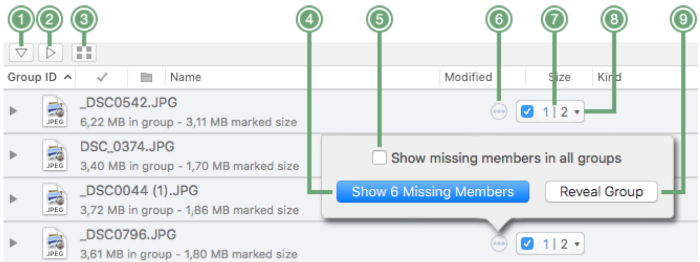
Figure 112: View by list details.
