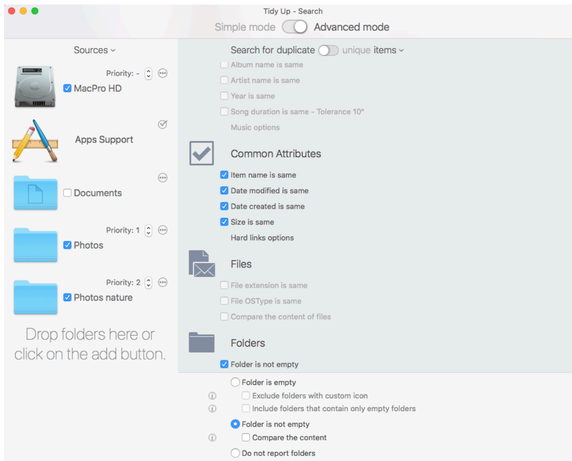
Figure 69: Search for similar folders.
