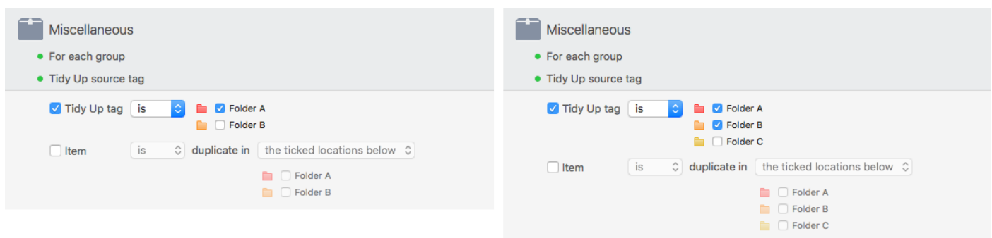
Figure 95: Remove all but one item of each duplicate group that resides in a specific location.
