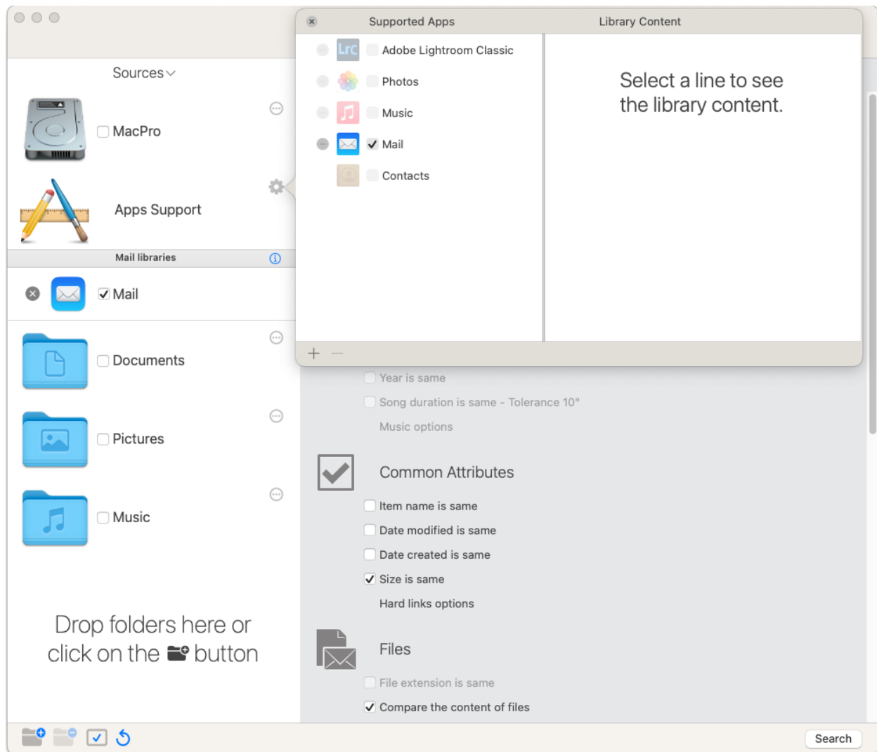
Figure 82: Search for duplicate e-mail messages in Mail.
