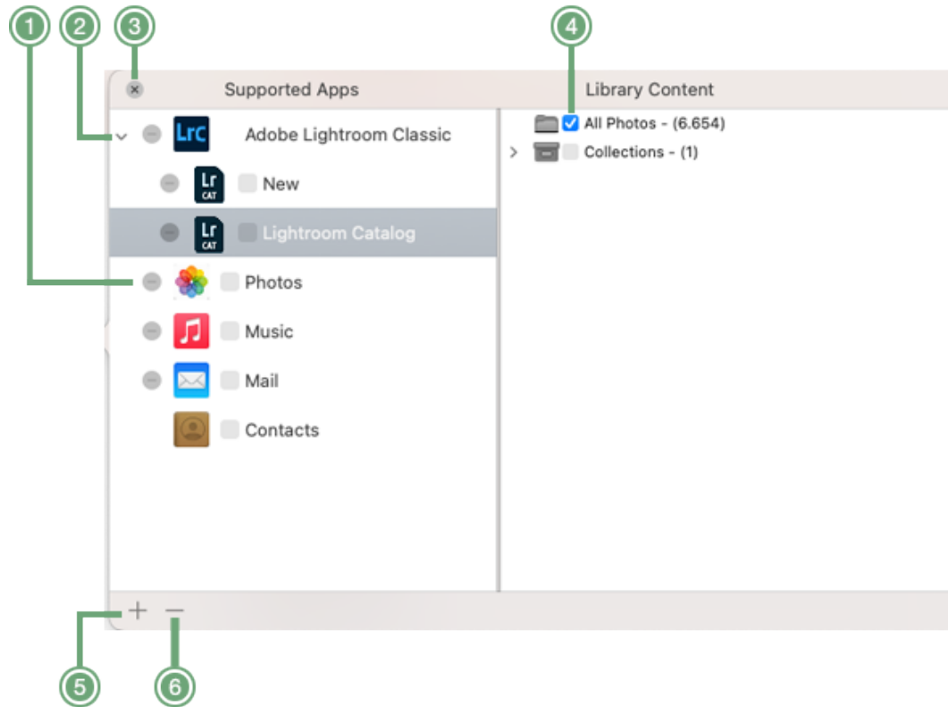
Figure 108: Apps support window.
