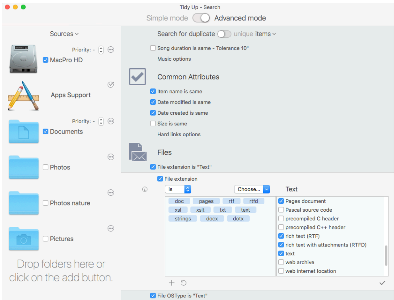
Figure 86: Search for similar text files.
