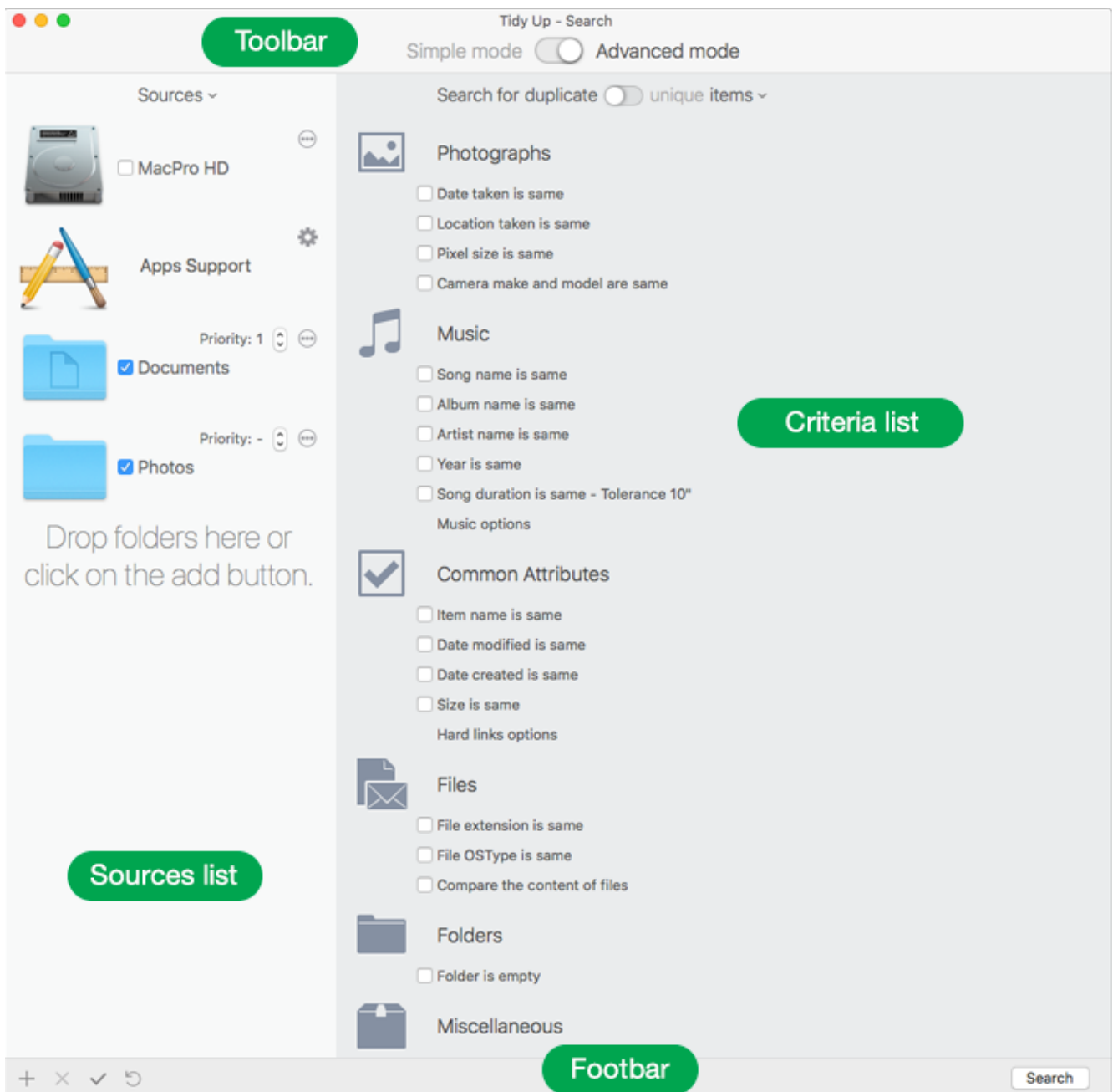
Figure 104: Search window – Advanced mode.
