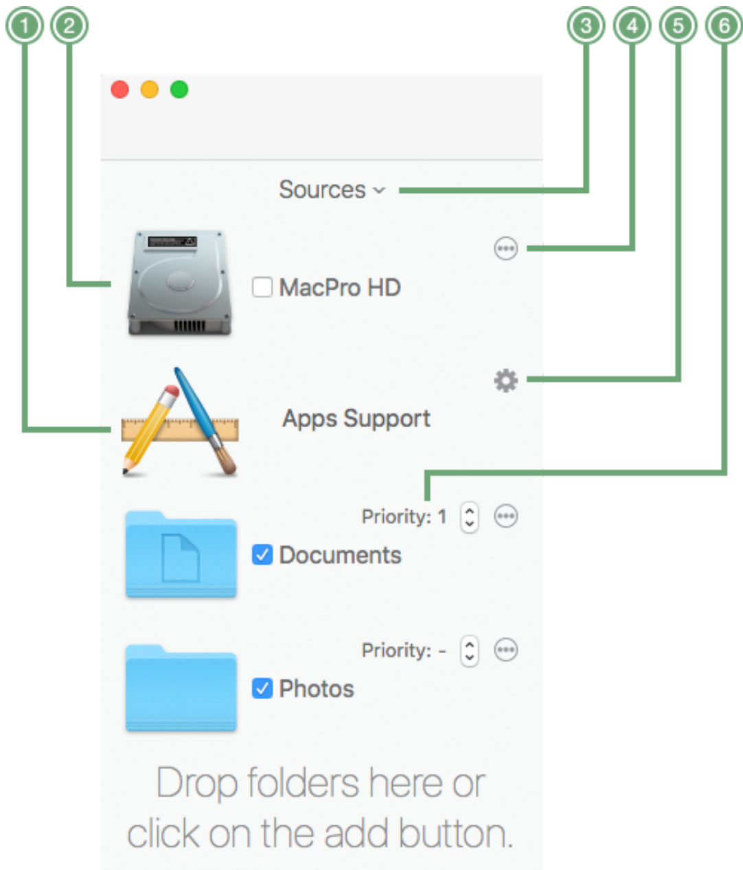
Figure 105: Search window – Advanced mode sources details.
