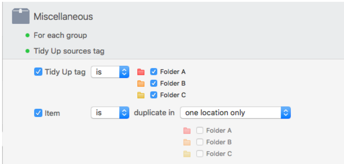
Figure 98: Remove all but one item of each duplicate group that reside in a specific location, but only if they are duplicates in a location only.
