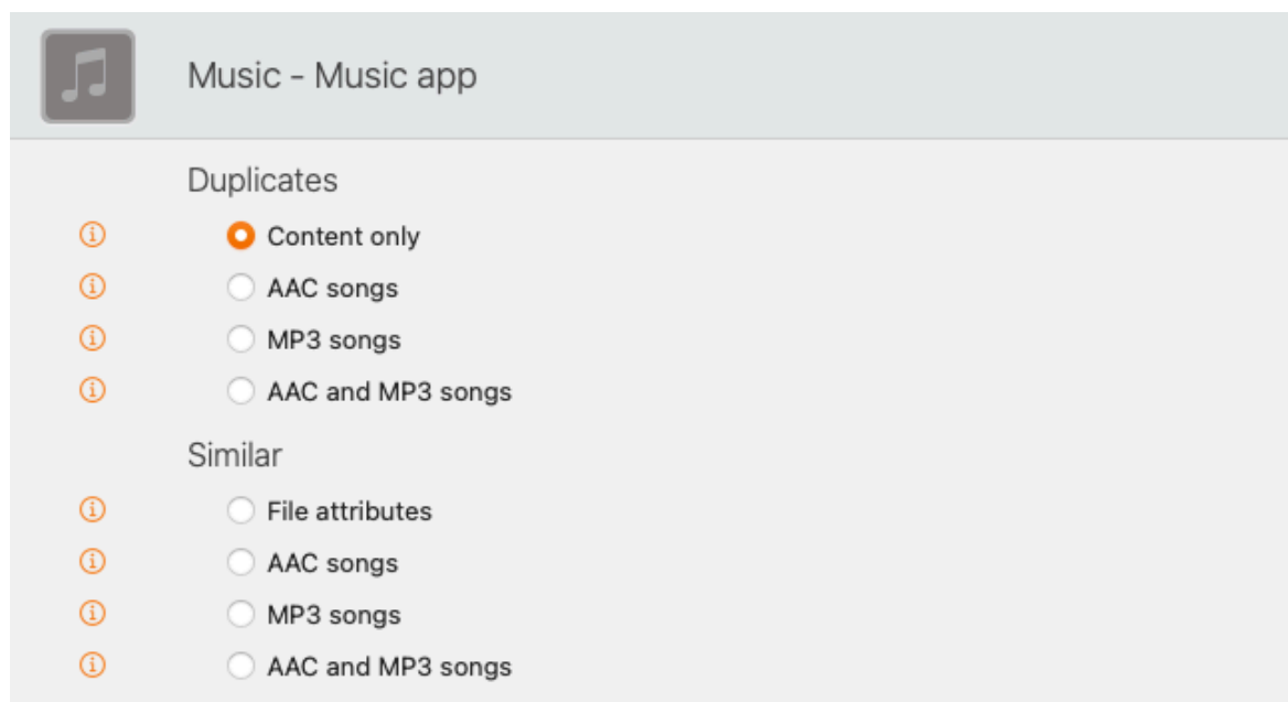
Figure 15: Music music search pane.
