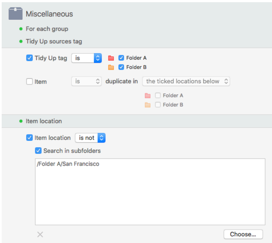
Figure 100: Remove all but one item of each duplicate group that reside in a specific location, but exclude a location within that location.
