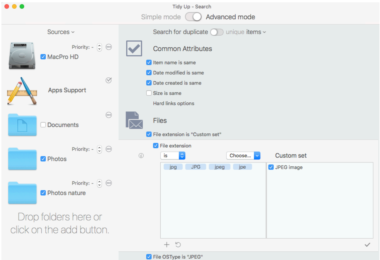
Figure 79: Search for similar JPEG images.
