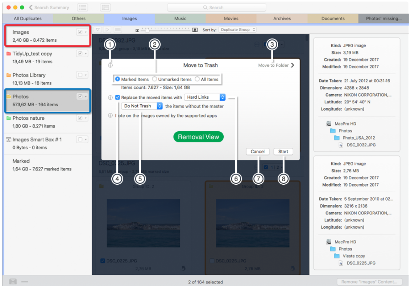
Figure 58: Remove view.
