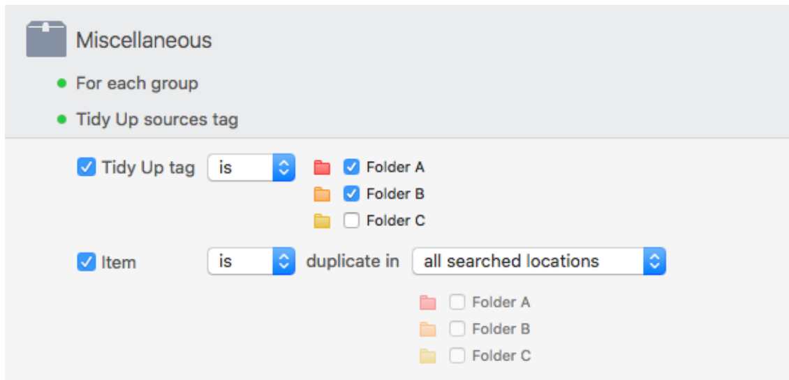
Figure 99: Remove all but one item of each duplicate group that reside in a specific location, but only if they are duplicates in all locations.
