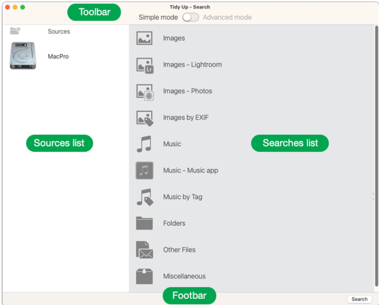
Figure 101: Search window – Simple mode.
