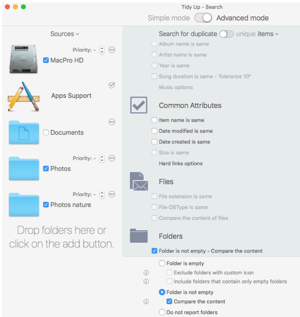
Figure 72: Search for duplicate folders by content.
