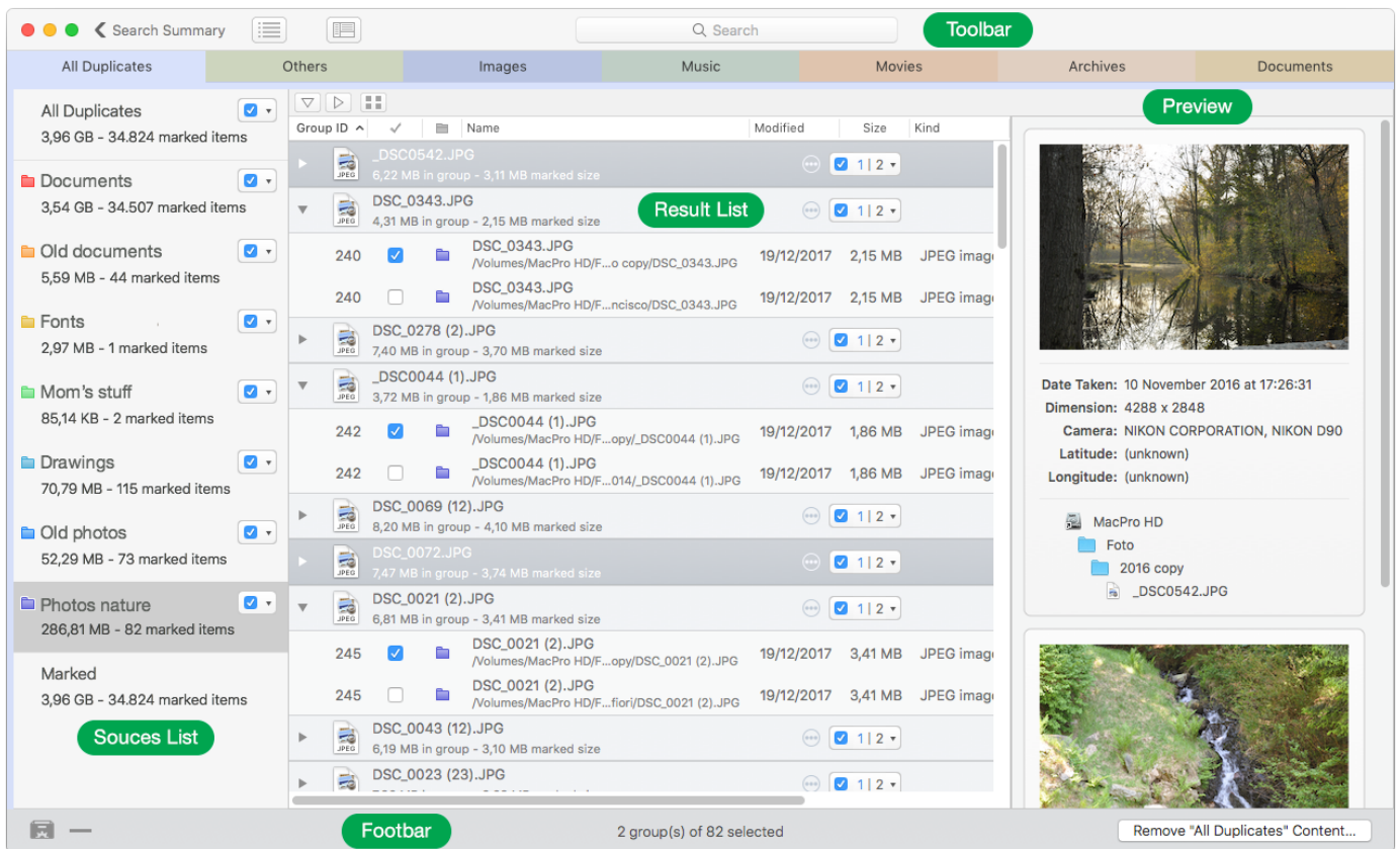
Figure 109: Result window.
